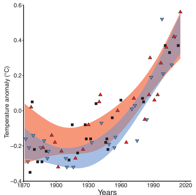
Fig. 1. Global warming throughout ENSO cycles. Sea surface temperature anomalies from 1871 to 2016,
